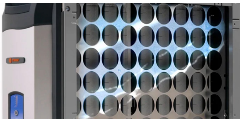
A cut-away of the Trane CleanEffects filter showing the field charger and reusable cells
